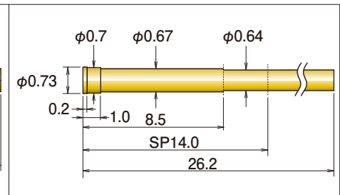
K2-0.48S-4-26.2L-2 (S048-140-05)
