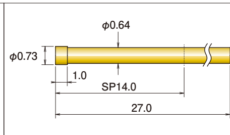
K2-0.48S-3-2 (S048-140-04)
