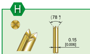
K2-0.26 III H-2M-1
