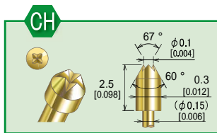
K2-0.26 III CH-4.5M0.3-4
