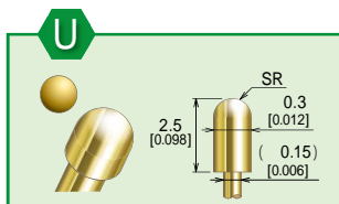
K2-0.26 III U-4.5M0.3-1
