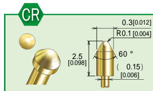
K2-0.26 III CR-4.5M0.3-3
