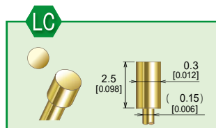
K2-0.26 III LC-4.5M0.3-1
