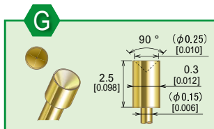
K2-0.26 III G-4.5M0.3-1
